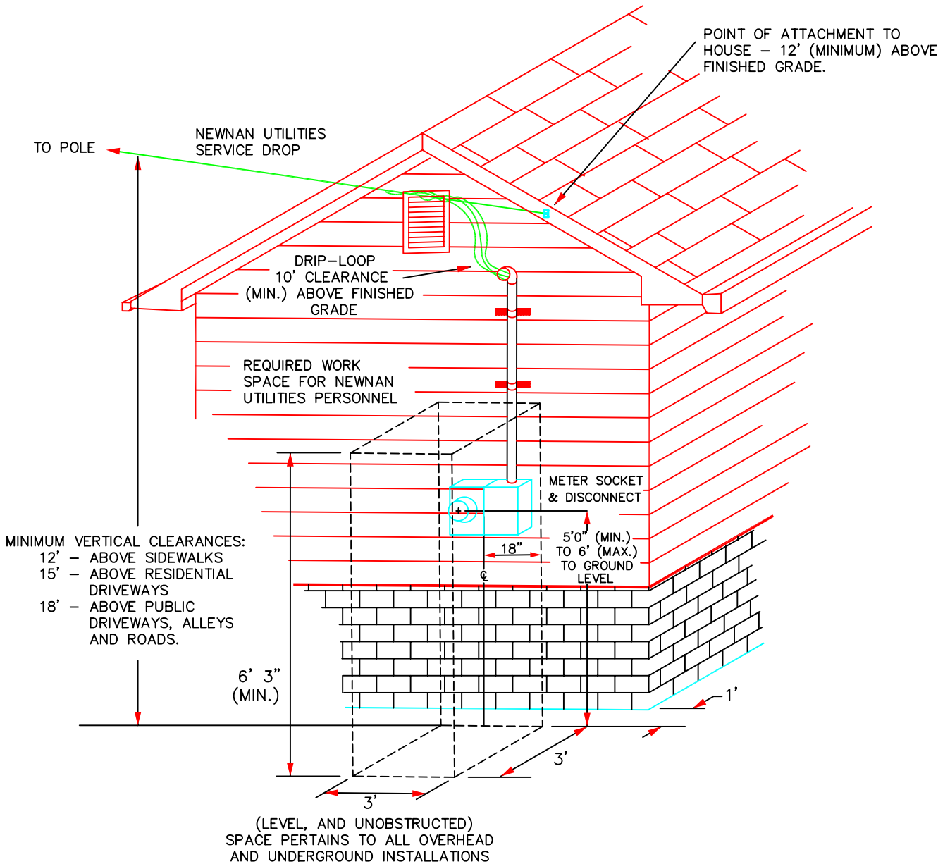
TYPICAL RESIDENTIAL OVERHEAD INSTALLATION
